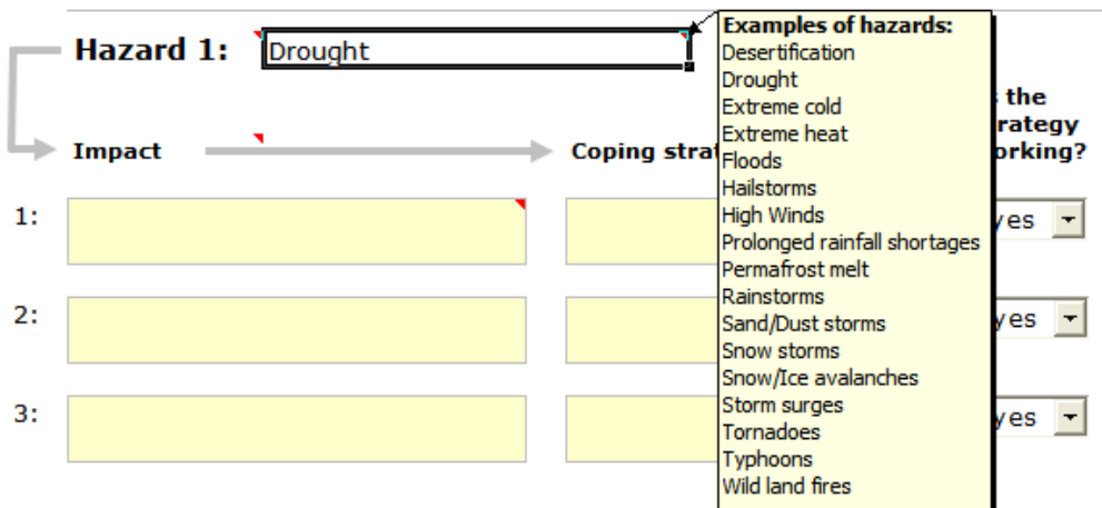
Figure 2-4: Examples of climate-related hazards
