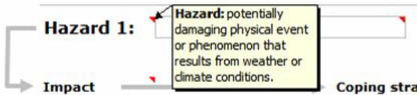
Figure 2-3: Definition of 'Hazard'
