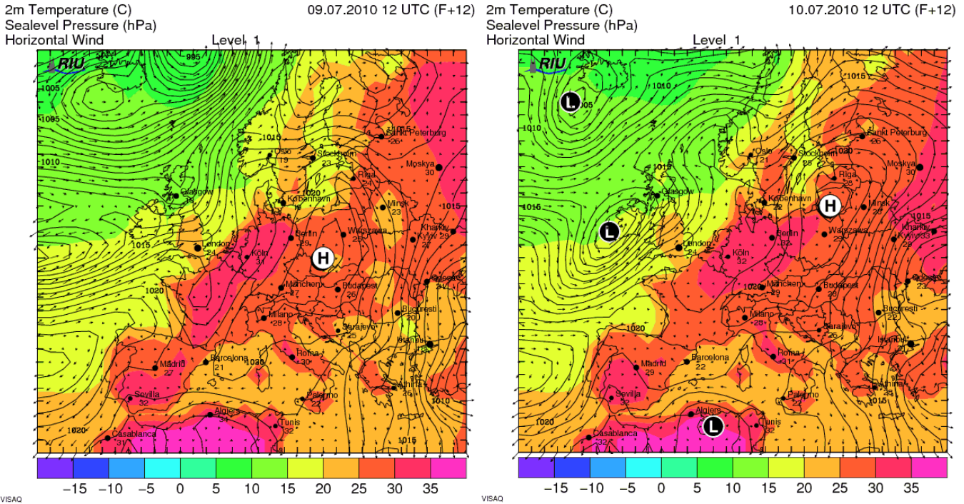
Map 2.3 Selected days during the summer 2010 ozone episodes: observed maximum 1-hour ozone concentrations and meteorological situation (cont.)
