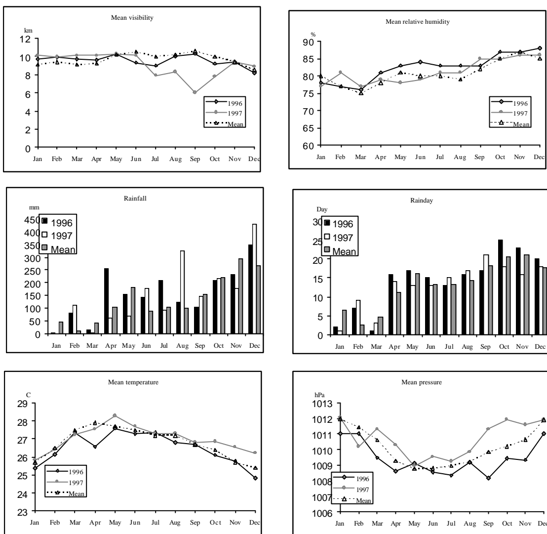
Figure 2 Monthly surface meteorological observations for Hat Yai in 1996 and 1997 compared with the 30-year mean
