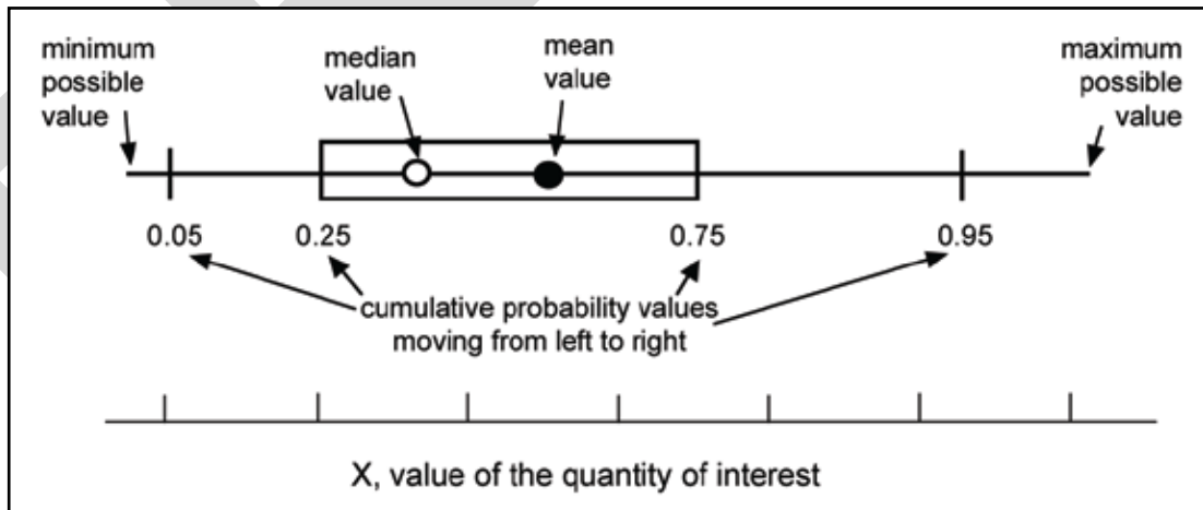
Figure 9.3 Recommended format for box plot. When many uncertain results are to be reported, box plots can be stacked more compactly than probability distributions.
