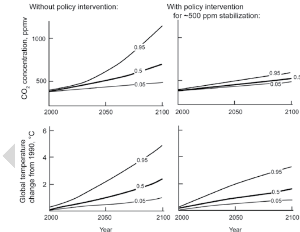
Figure 6.2 Results of simulation conducted by Webster et al. (2003) that use an earlier version of the MIT IGSM model with probability distributions on model inputs that are constrained by past performance of the climate system. Results on the left are the authors' projection for no policy intervention and on the right for a specific policy intervention that roughly achieves stabilization at 500 parts per million by volume (ppmv). Heavy curves show median results from the simulations. Light curves show 0.05 and 0.95 confidence intervals. [Redrawn from Webster et al. (2003).]
