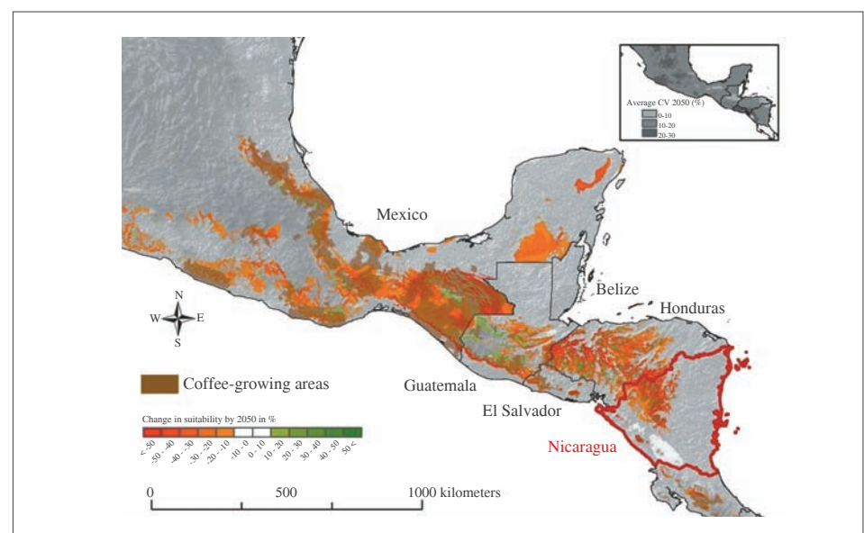
Figure 1. Projected changes in suitability in Mesoamerica by 2050 and coefficient of variance of 18 different Global Circulation Models (GCM) used for the analysis (small map).
