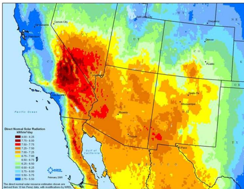
Figure 2: Solar Intensity in the Southwest
