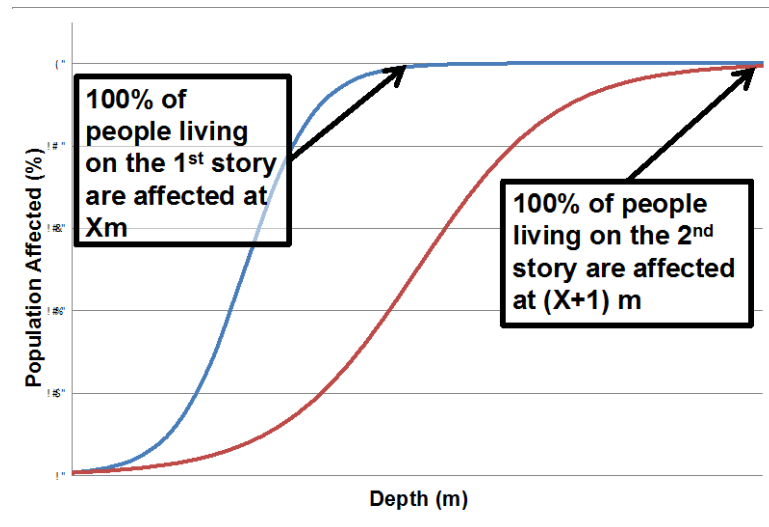
Figure A.5 Depth damage curves provide a relationship between depth and the percent of the population affected, based on building story.
