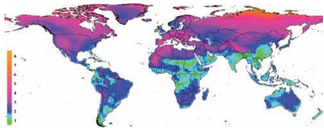
National Centre for Atmospheric Research (NCAR), wettest scenario
