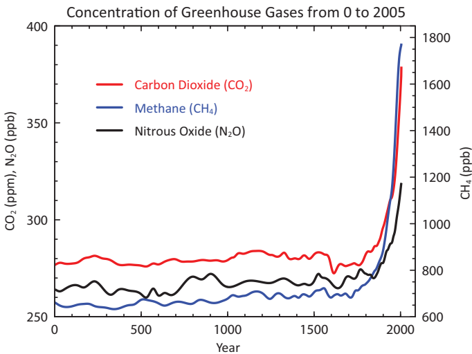
FAQ 2.1, Figure 1 (Errata). Revised figure showing atmospheric concentrations of important long-lived greenhouse gases over the last 2,000 years. Using the combined and simplified data from Chapters 6 and 2, the original figure displayed the CH 4 curve incorrectly. The revised figure shows the same data correctly plotted. For further details please refer to the original figure caption.
