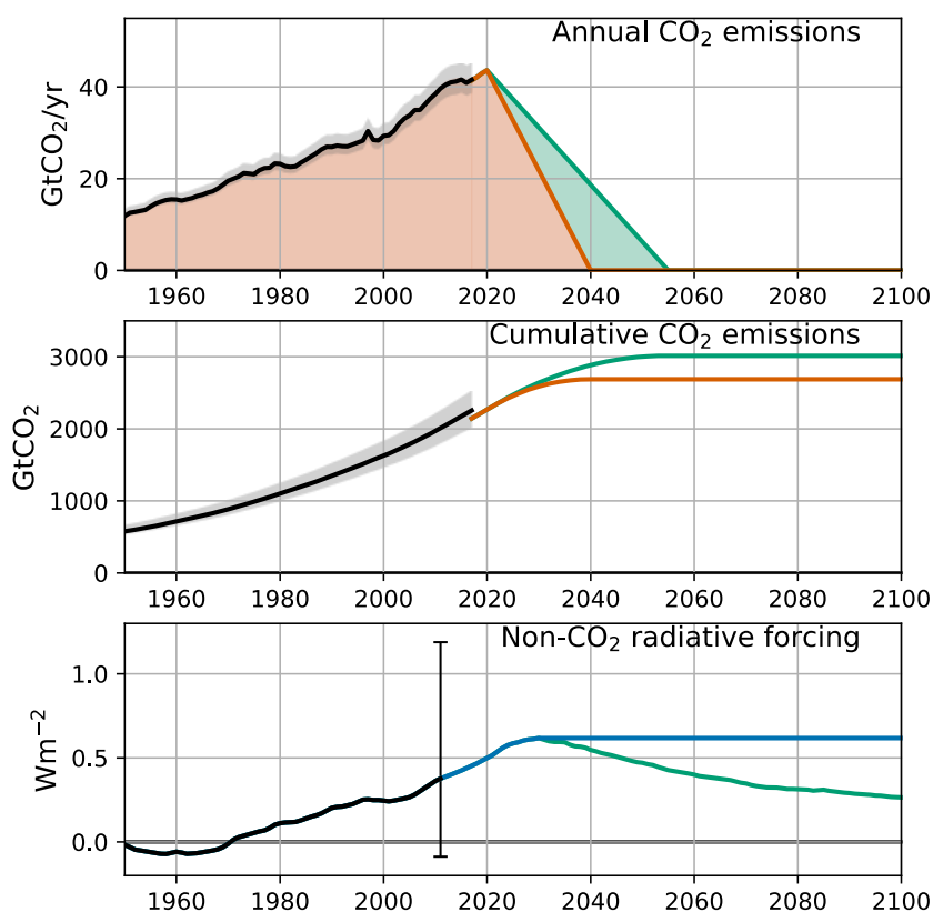
Technical Annex 1.A, Figure 11: Time-series of (top) annual CO 2 emissions, (middle) cumulative CO 2 emissions, and (bottom) non-CO 2 radiative forcing corresponding to observation-based estimates over the historical period and idealised 1.5°C-consistent pathways.
